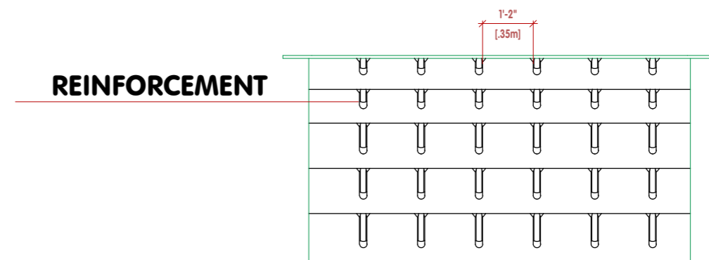
CROSS SIDE VIEW D-D
