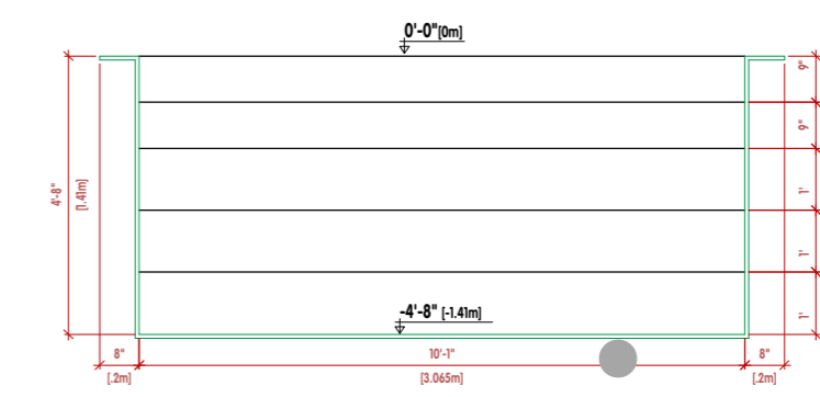
CROSS SECTION B-B
